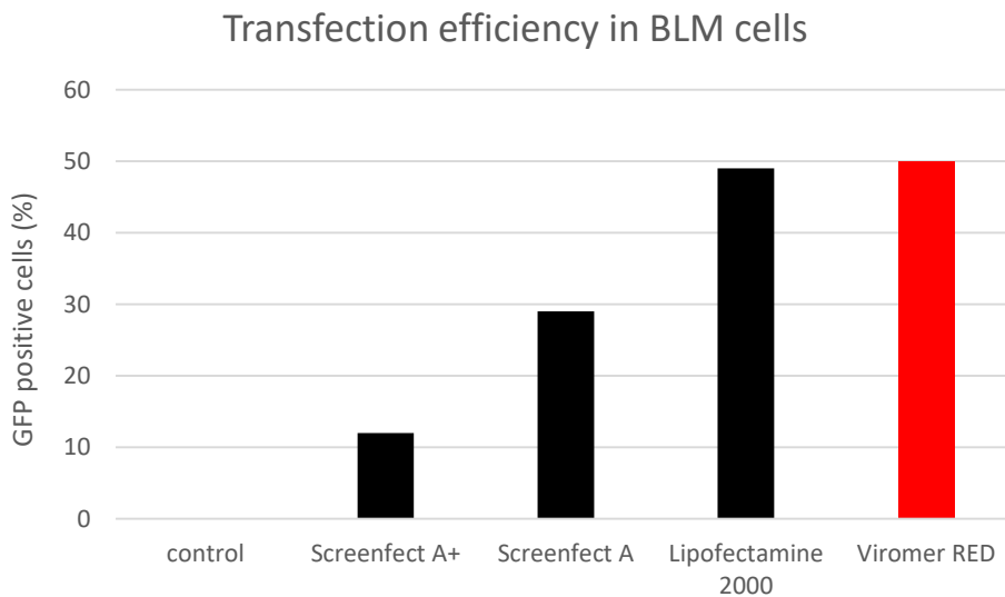
Fig. 1: Comparative GFP expression in BLM cells (melanoma cells) transfected with Viromer® RED, Screenfect A/A+ and Lipofectamine® 2000
